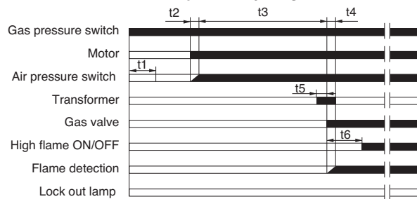
Normal operative cycle ignition
