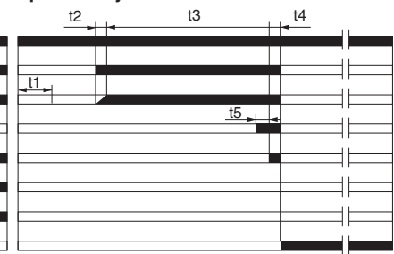
Operative cycle with flameless
