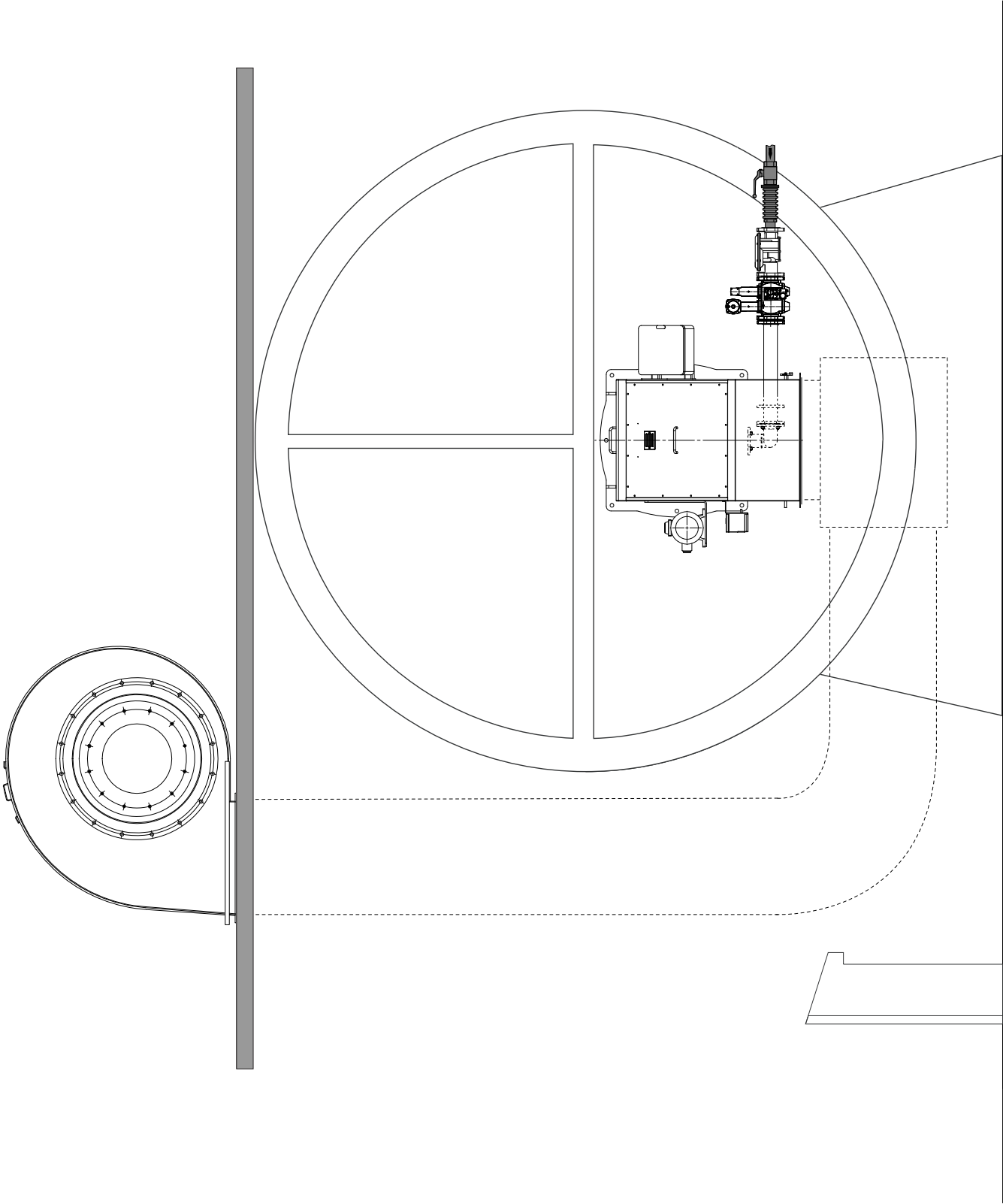
OVERALL DIMENSIONS MULTICALOR 2000.1 MD LMV TS
