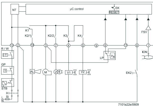
Connection diagram and control sequence of LME21...
